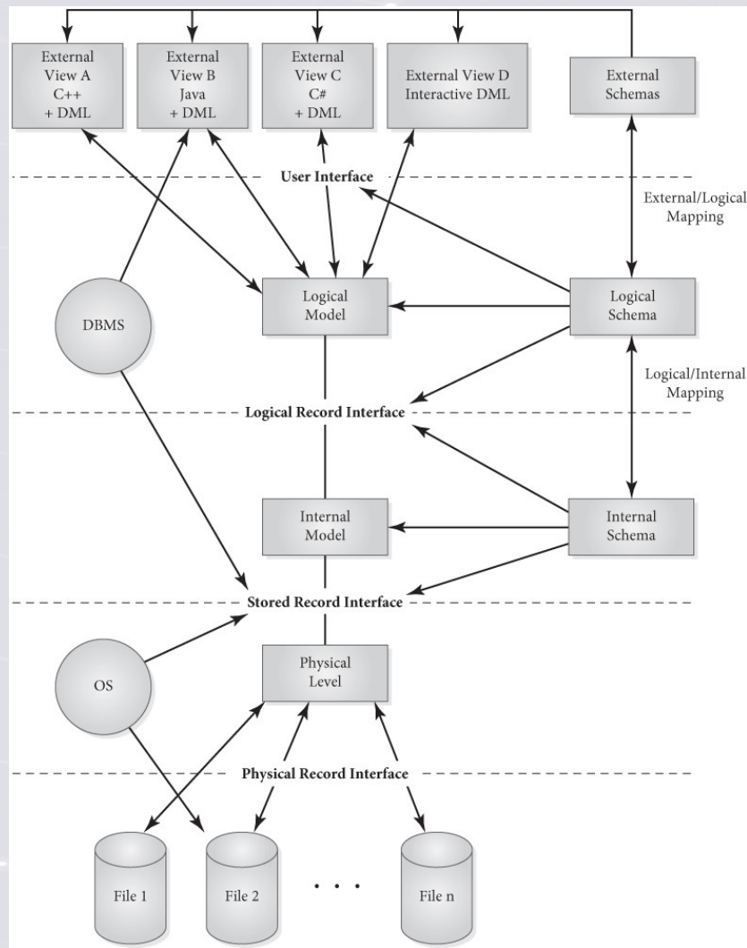
Figure 02.F04: Three-Level Database Architecture
