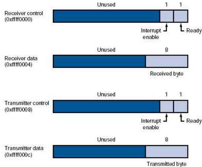
Figure 7: The terminal is controlled by four device registers, each of which appears as a special memory location at the given address. Only a few bits of the registers are actually used: the others always read as zeroes and are ignored on writes.
