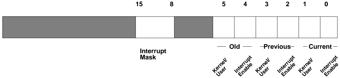
Figure 3: The Status register.
